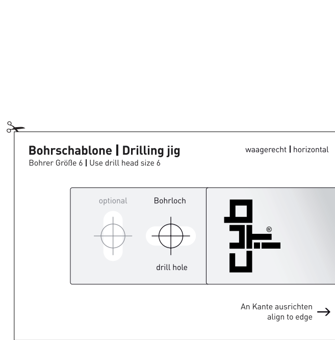
Drilling jig for horizontal alignment
